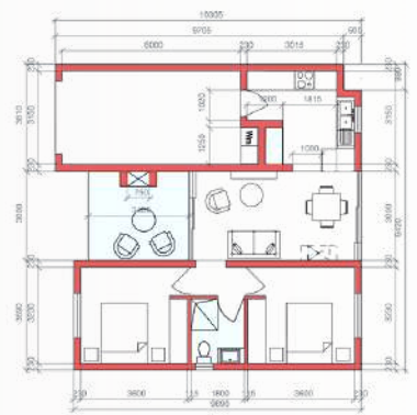
Unit Type 2 1:100 70sqm House 20sqm Garage 10sqm Pergola
