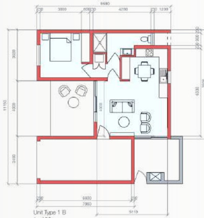
Unit Type 1 B 1:100 60sqm House 24sqm Garage 10sqm Pergola
